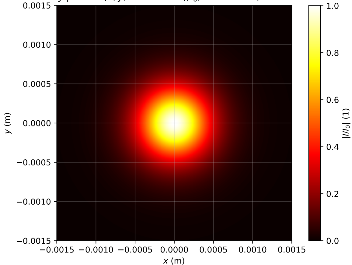
Intensity profile I(x, y, z = 2.388m)/I_0 , P_{in}=0.7P_{cr} , artificial time
